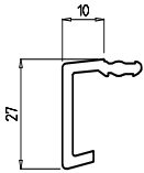
Fensterbankabdeckung 27 x 10 mm Art.-Nr. 559
